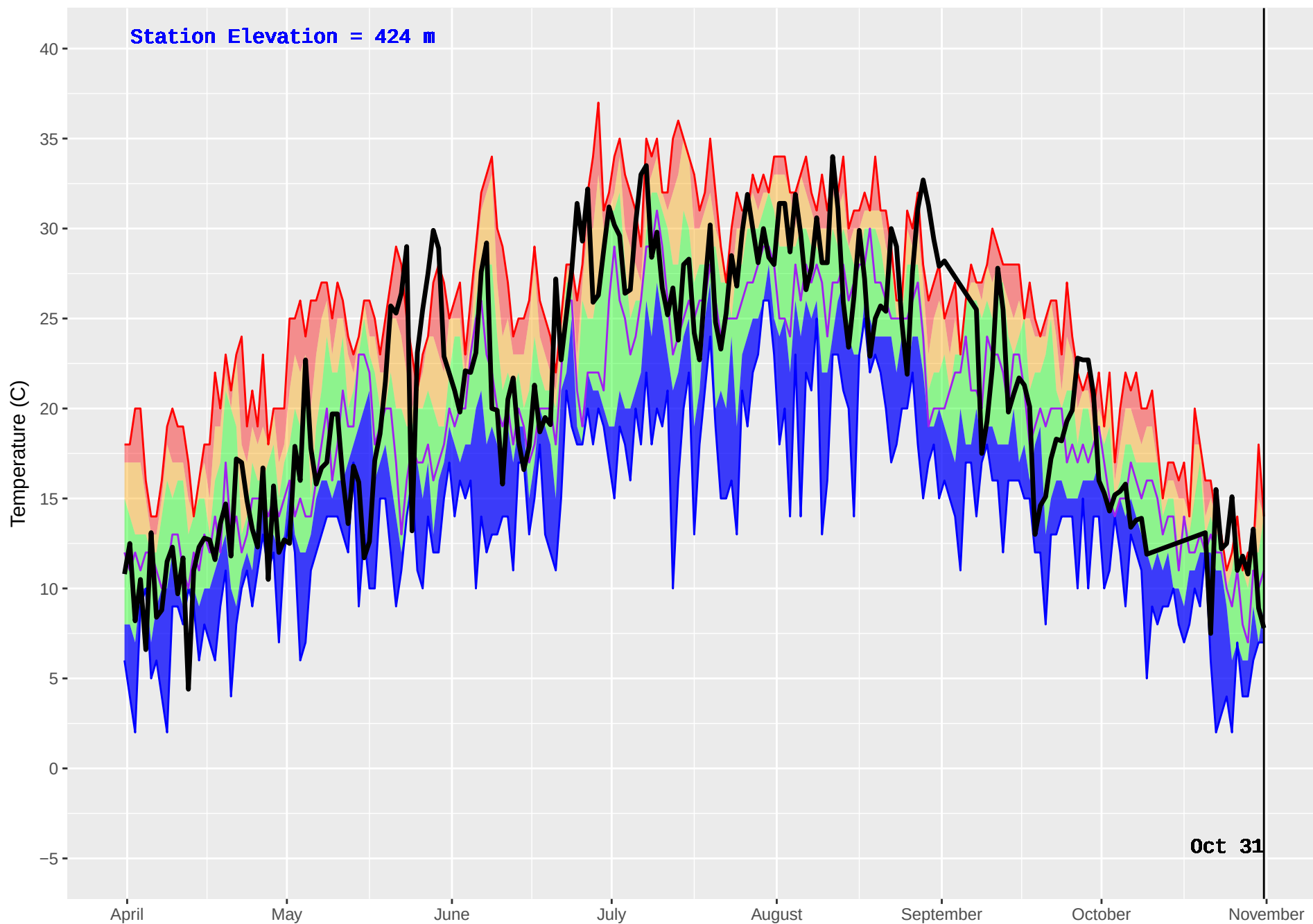
SPLINTLUM (1055) : Historical (2009–2016) and Current (2017) Noon Temperature
