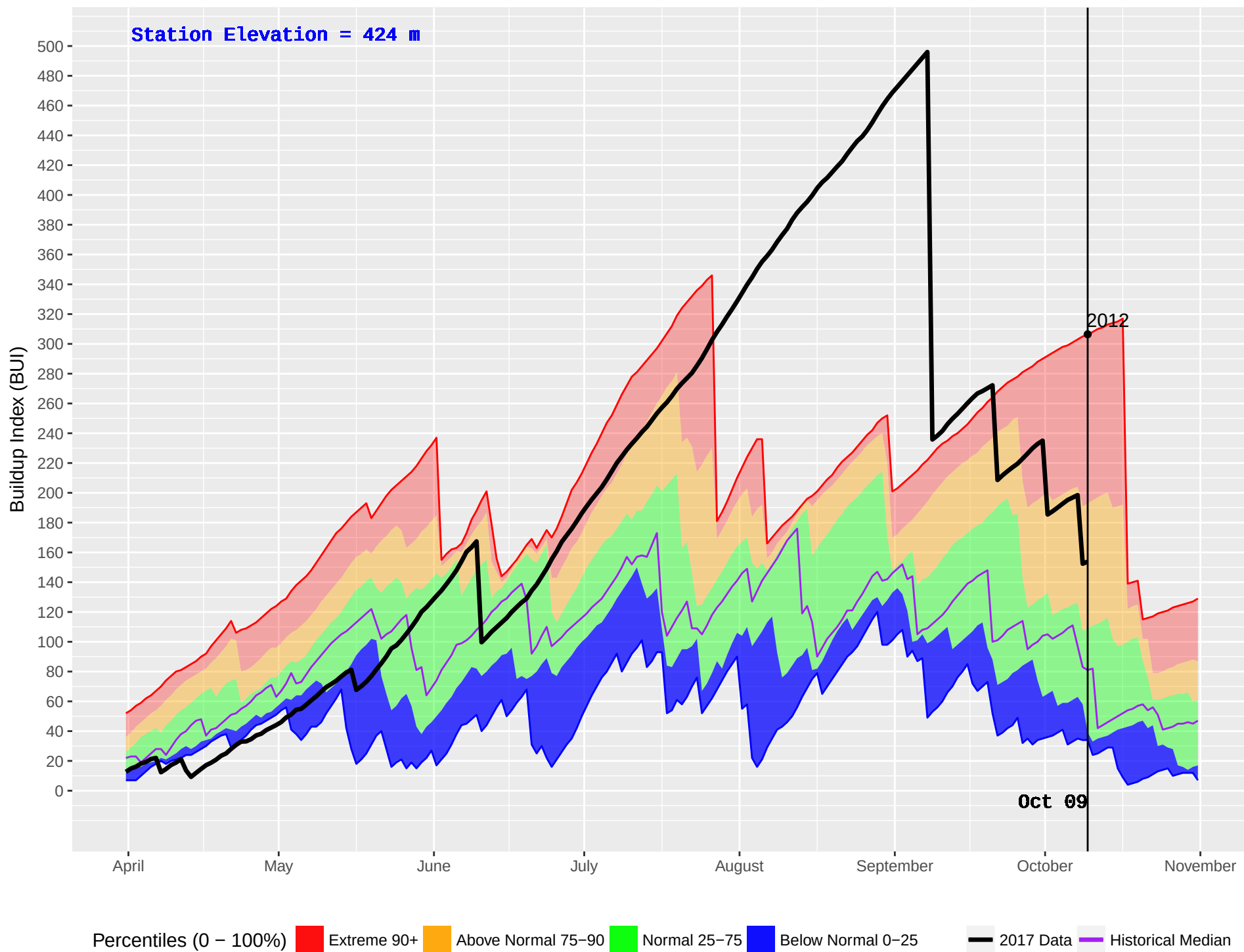
SPLINTLUM (1055) : Historical (2009–2016) and Current (2017) Noon Buildup Index (BUI)
